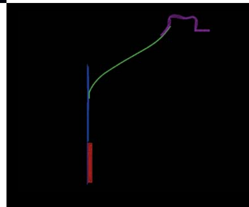
Figure 11. The shape of the first mode with a C.M.M.D. cone, at 10,190Hz.
