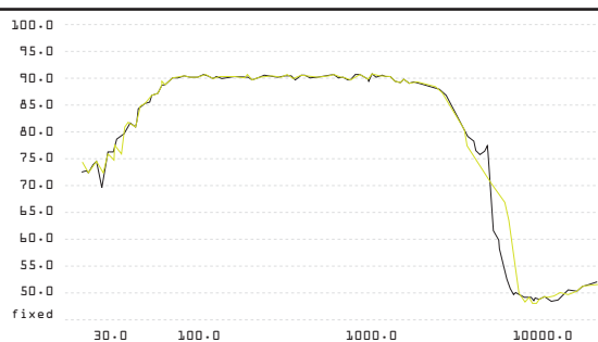
Figure 13. When the attenuation of the crossover network is added to the curves of Figure 12, the result is that, in the C.M.M.D. cone, the amplitude of the first bending resonance is about 10dB lower than that in the aluminum cone – this is not a trivial improvement. The final frequency-response curve approaches the theoretical ideal very closely indeed, even far beyond the crossover frequency.
