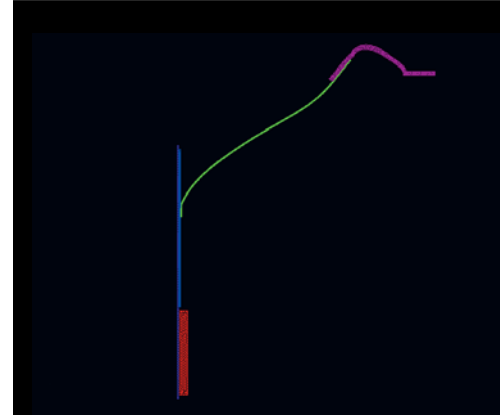
Figure 7. The shape of the first mode with a paper cone, at 2160Hz.
