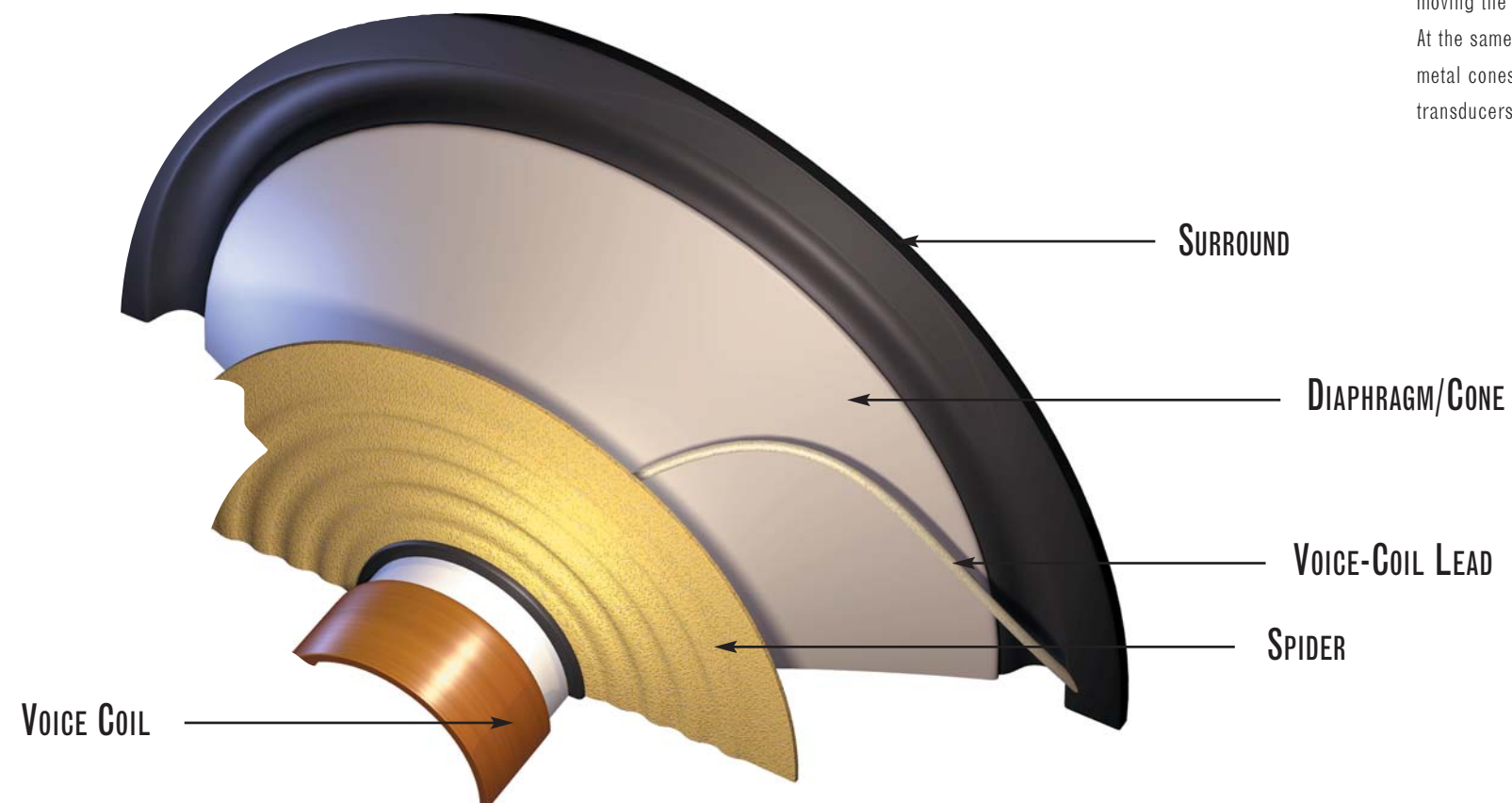
Figure 1. The construction of a cone assembly, showing the diaphragm connected to the voice coil that drives it, and spider and surround that support it.
