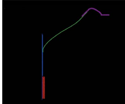
Figure 6. The shape of the first mode with a Kevlar fabric composite cone, at 1920Hz.
