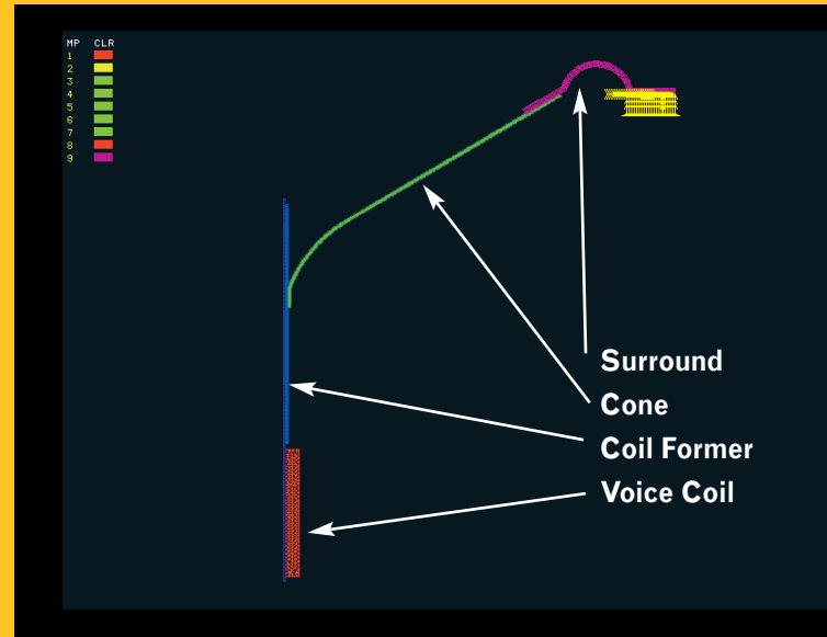
Figure 3. This shows a radial slice through the cone assembly. It shows the voice coil (red), the coil former (the vertical blue line), the cone (greenish), and the surround (purple) attached to the frame.
