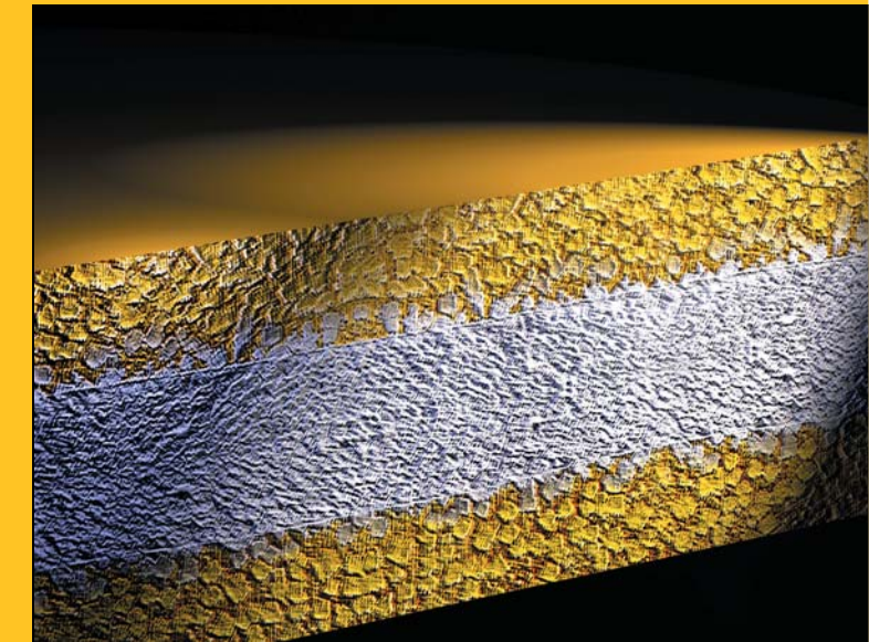
Figure 4b. An electron microscope photograph showing a cross section of a C.M.M.D. cone.
